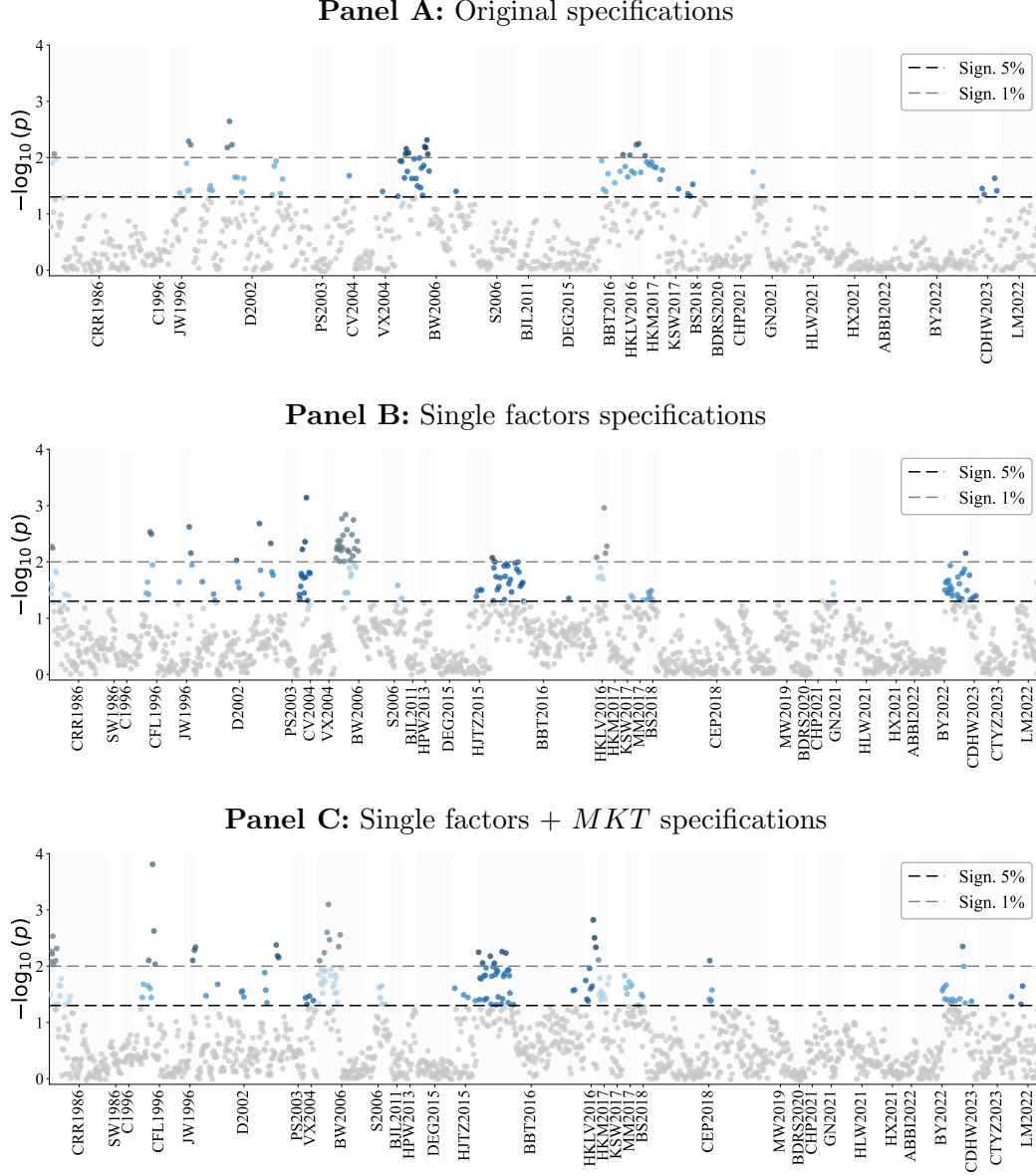
Figure B.8: Significance of portfolio premia from \beta -sorted portfolios across papers. This figure plots the -\log_{10}(p\text{-value}) from tests of whether average long-short portfolio expected returns differ from zero for the original specifications (Panel A), single-factor models (Panel B), and single-factor models augmented with the market factor (Panel C). Higher values indicate stronger statistical significance. The labels follow the factor definitions presented in Tables A.1–A.5.
